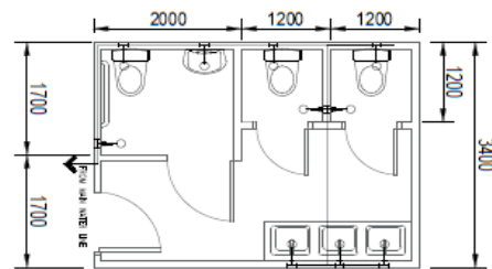
WATERLINE LAYOUT PLAN
