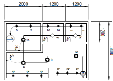
LIGHTING LAYOUT PLAN
