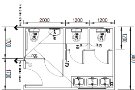
SEWER & DRAINAGE LAYOUT PLAN
