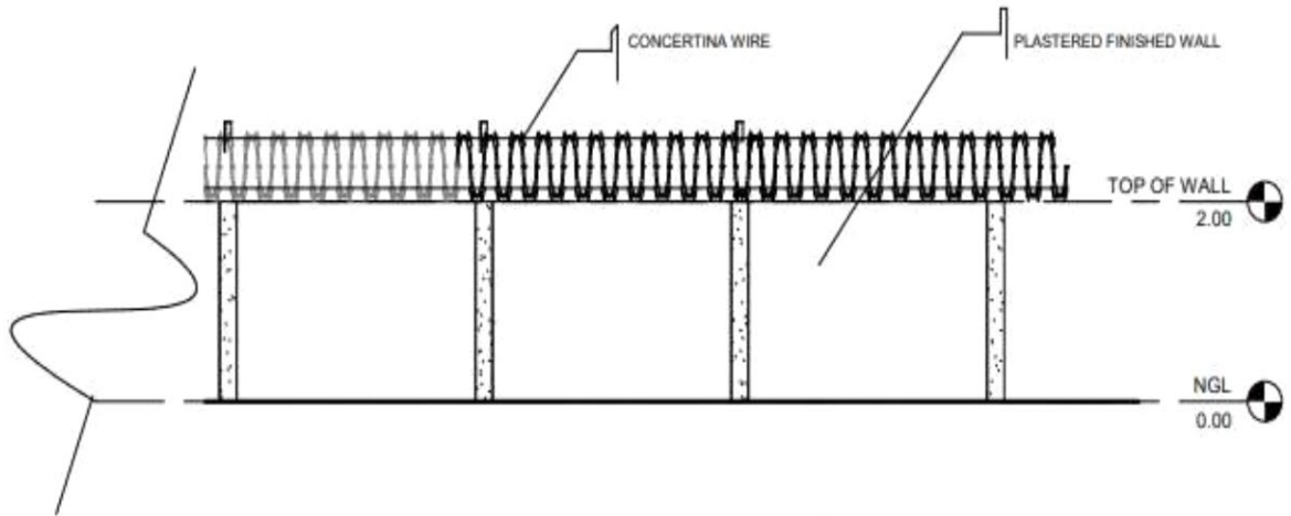
2 WALL ELEVATION 1 : 50
