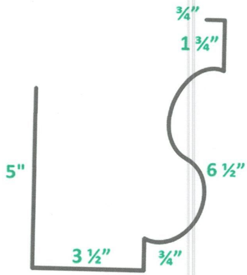
SPANISH GUTTER 18"
