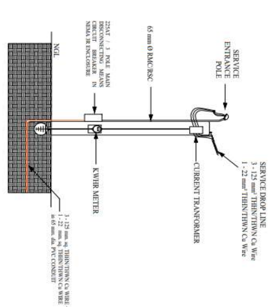
SERVICE ENTRANCE EQUIPMENT & GROUNDING
