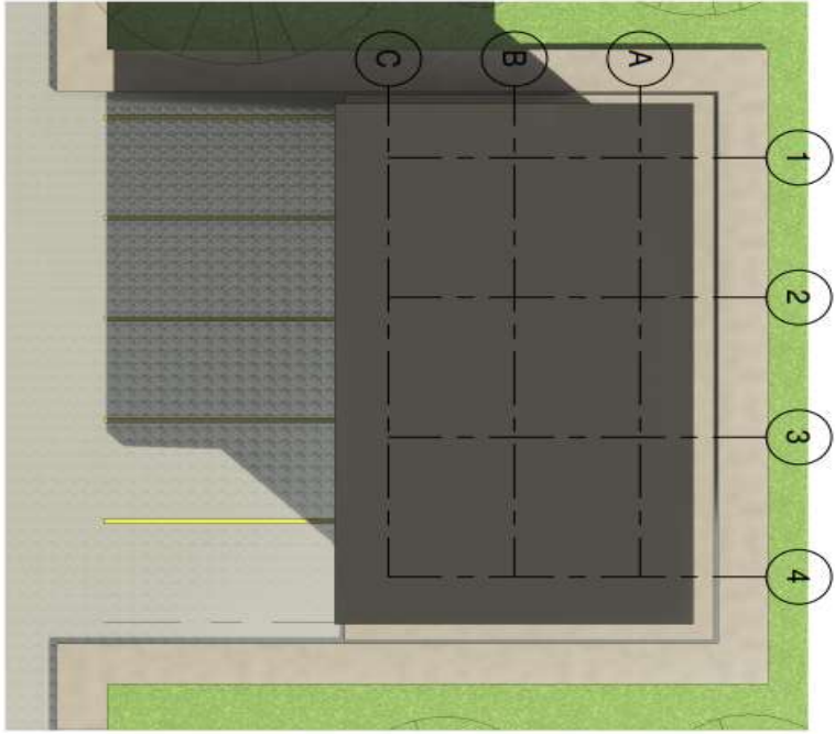
1 SITE DEVELOPMENT PLAN SCALE 1 : 100
