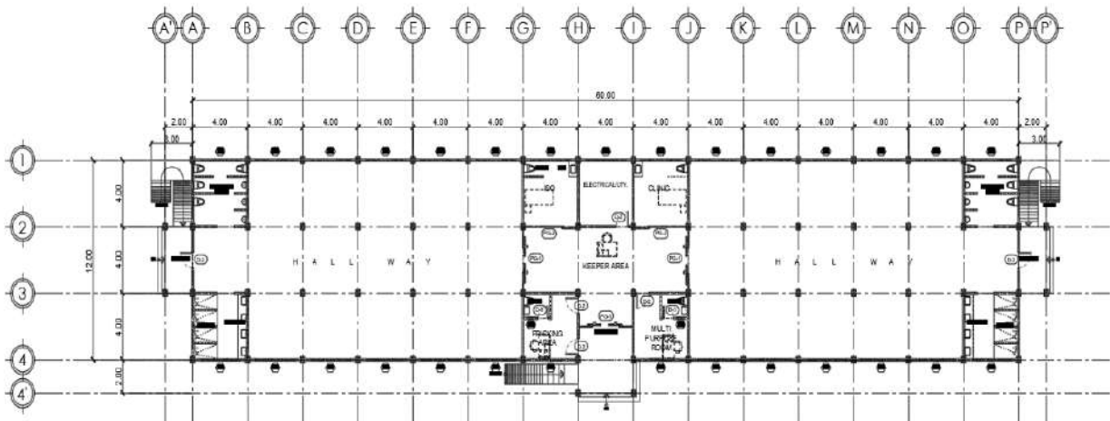
FLOOR PLAN
